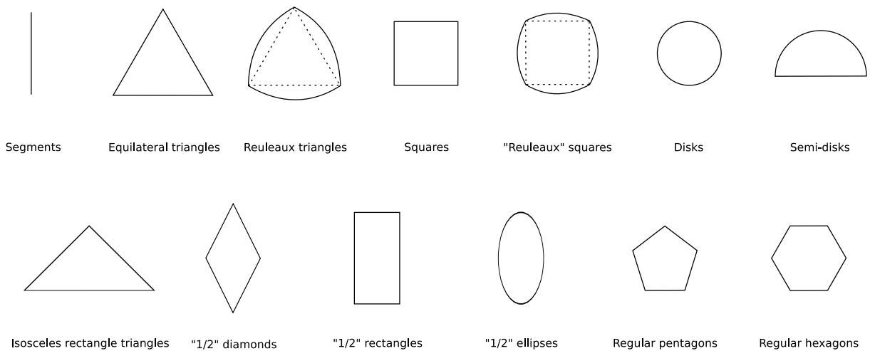
Figure 3: Family \mathcal{F}_1^c of 2D analytic compact convex sets.
