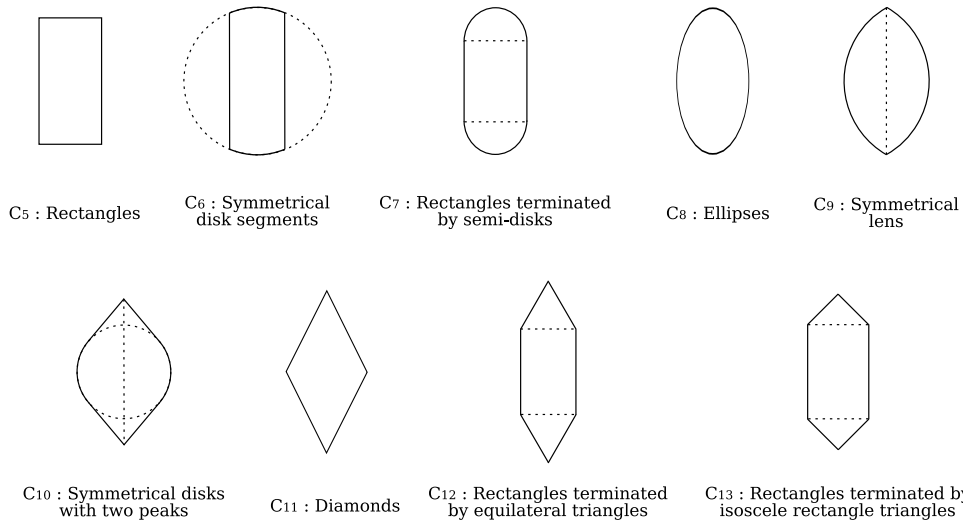
Figure 9: Family \mathcal{F}_{2,2}^c of 2D analytic compact convex sets with one degree of freedom and two symmetrical axes.
