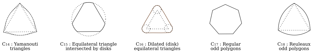
Figure 10: Family \mathcal{F}_{2,3}^c of 2D analytic compact convex sets with one degree of freedom and an odd number (strictly greater to 1) of symmetrical axes.
