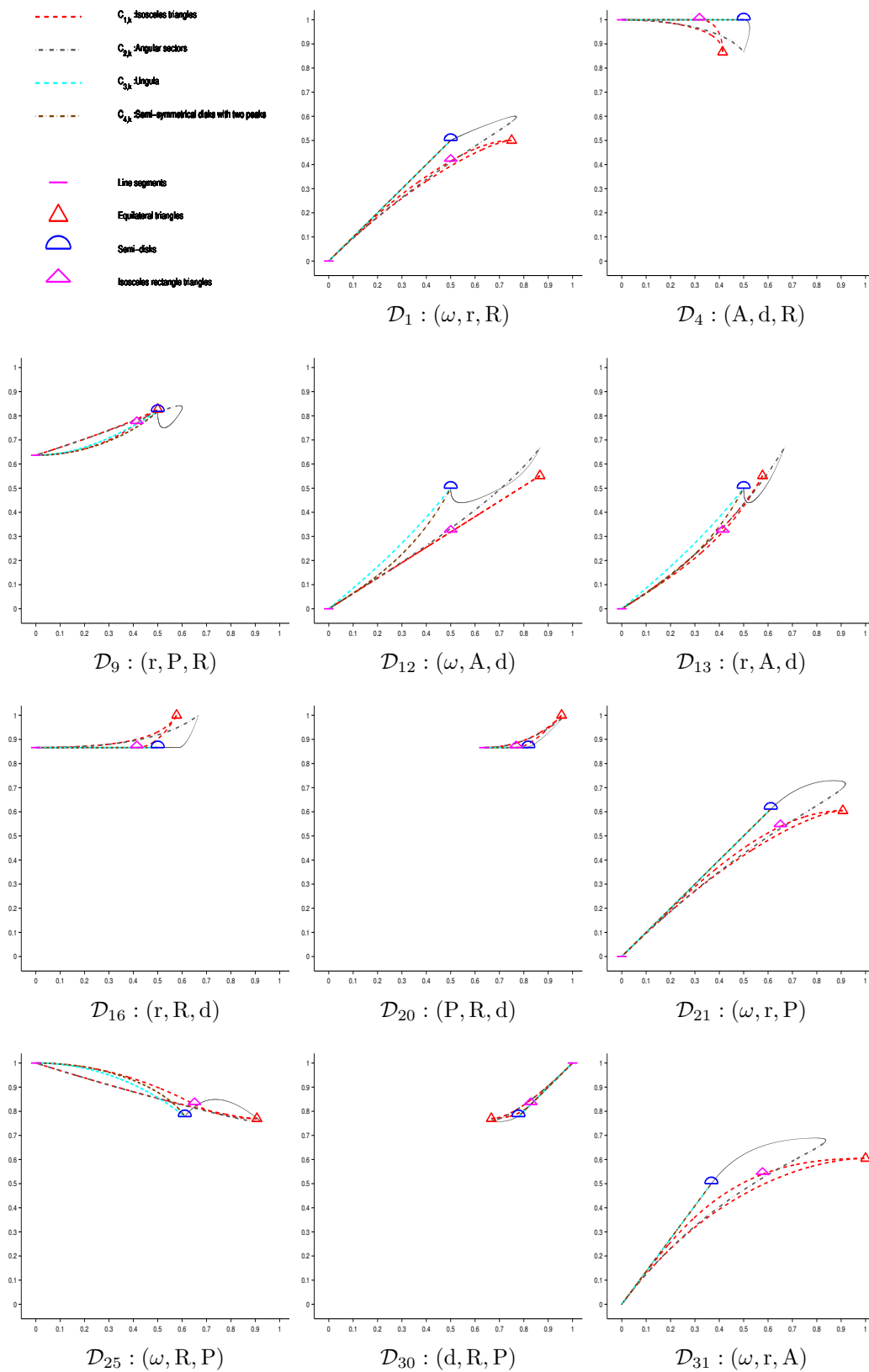
Figure 12: Family \mathcal{F}_{2,1}^c of analytic compact convex sets with one degree of freedom and one symmetrical axis mapped into eleven shape diagrams (chosen according to the results synthesized in section 6).
