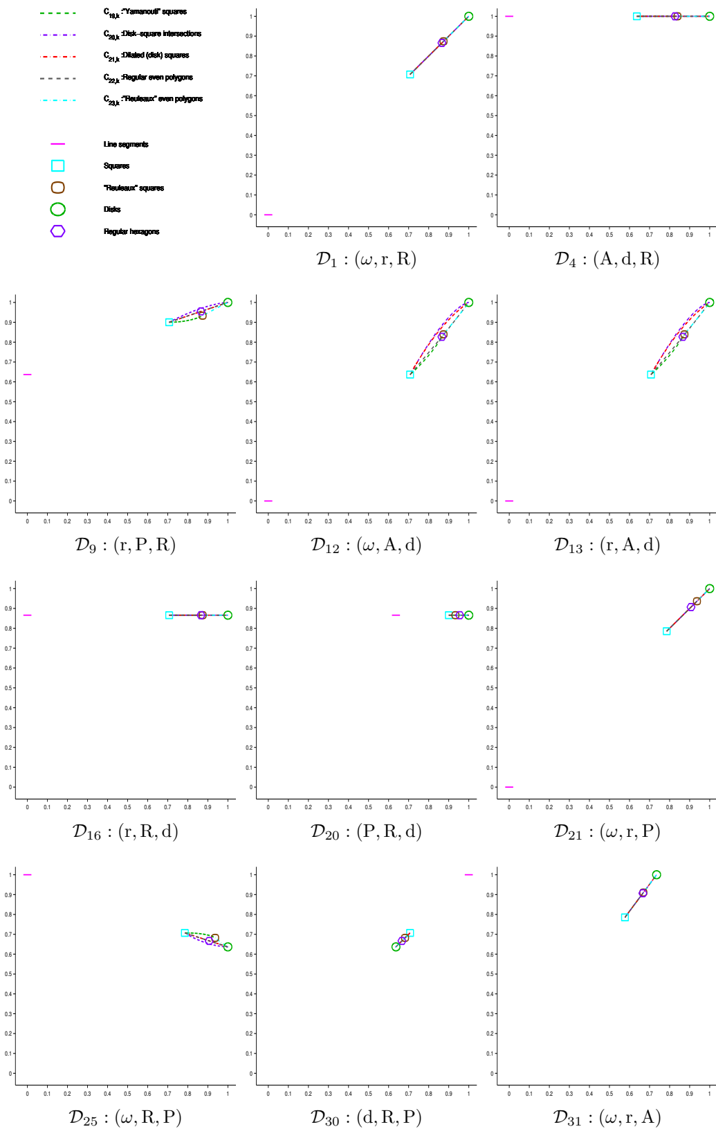
Figure 15: Family \mathcal{F}_{2,4}^c of analytic compact convex sets with one degree of freedom and an even number strictly greater to 2 of symmetrical axes mapped into eleven shape diagrams (chosen according to the results synthetized in section 6).
