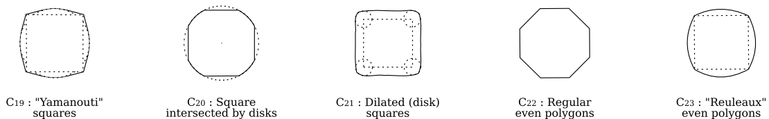
Figure 11: Family \mathcal{F}_{2,4}^c of 2D analytic compact convex sets with one degree of freedom and an even number (strictly greater to 2) of symmetrical axes.
