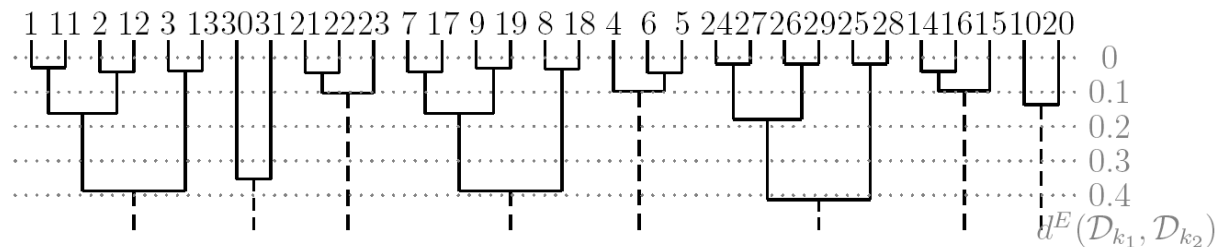
Figure 6: The firsts twenty-three steps of an algorithm of hierarchical classification based on distances between the shape diagrams. To each step, two shape diagrams are similar up to the distance values, whose the scale is indicated on the right.
