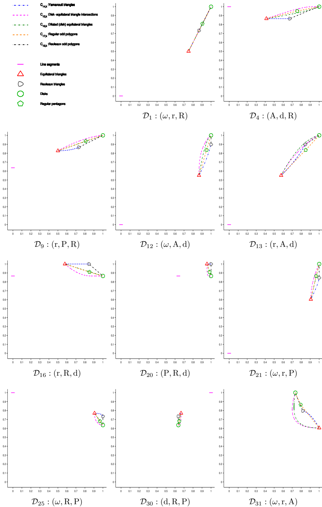
Figure 14: Family \mathcal{F}_{2,3}^c of analytic compact convex sets with one degree of freedom and an odd number strictly greater to 1 of symmetrical axes mapped into eleven shape diagrams (chosen according to the results synthesized in section 6).
