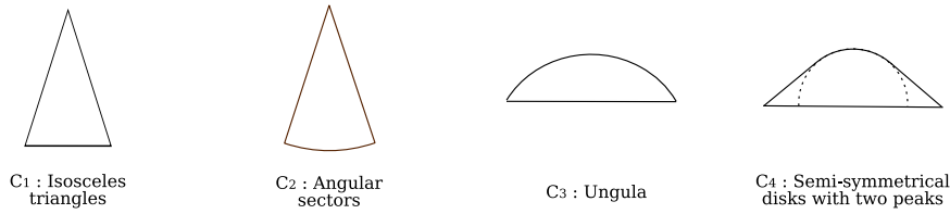
Figure 8: Family \mathcal{F}_{2,1}^c of 2D analytic compact convex sets with one degree of freedom and one symmetrical axis.
