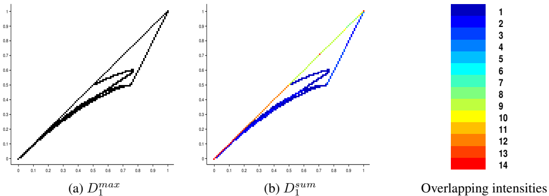
Figure 16: "Intensity" discretized shape diagram D_1 : (\omega, r, R) ( n = 100 ) with the twenty-three curves representing the compact convex set classes with one degree of freedom.
