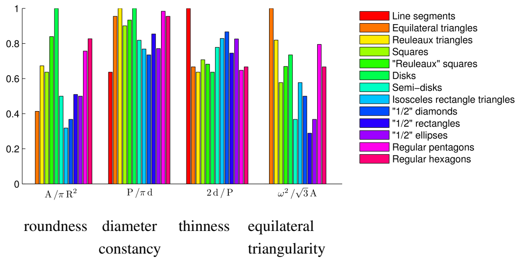
Figure 2: Values of several morphometrical functionals for elementary 2D compact convex sets.
