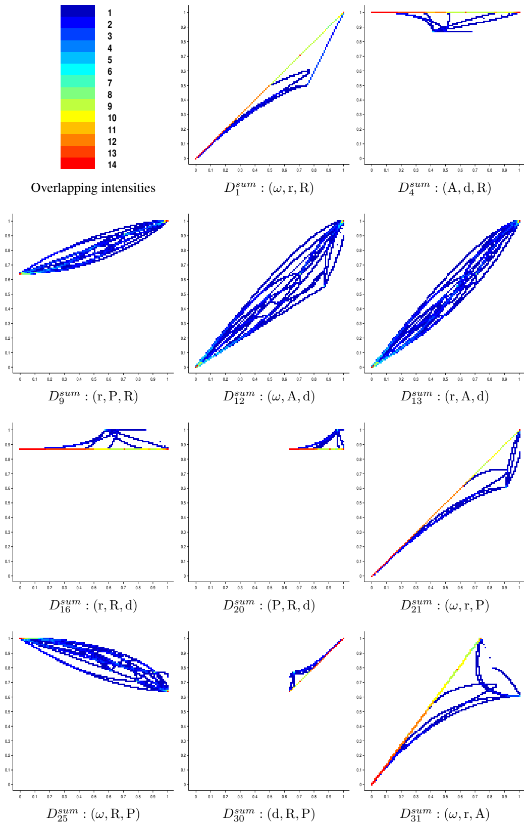
Figure 17: "Intensity" discretized shape diagram D_k^{sum} ( n = 100 ) with the twenty-three curves representing the compact convex set classes with one degree of freedom.
