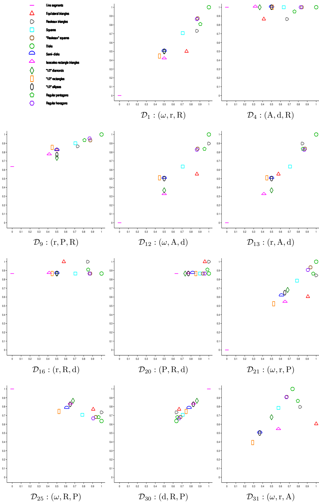
Figure 5: Family \mathcal{F}_1^c of analytic compact convex sets mapped into eleven shape diagrams (chosen according to the results synthesized in section 6).
