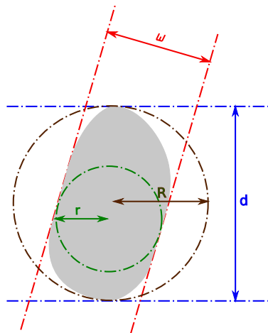
Figure 1: Geometrical functionals of a compact convex set: radii of inscribed ( r ) and circumscribed ( R ) circles, minimum ( \omega ) and maximum ( d ) Feret diameters.
