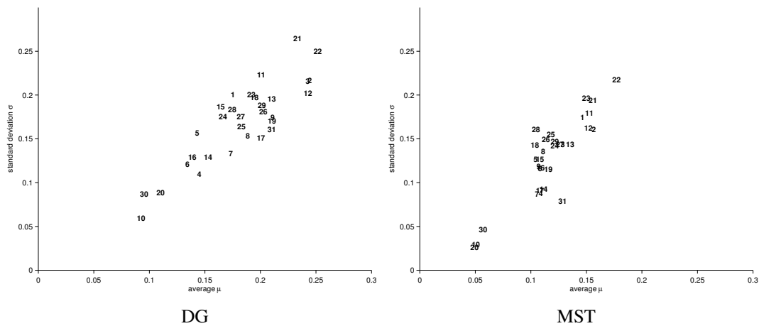
Figure 7: Two dispersion quantifications for all shape diagrams applied on the family \mathcal{F}_1^c . For each representation (according to the models DG and MST, respectively), indices k \in \llbracket 1, 31 \rrbracket of the shape diagrams \mathcal{D}_k are located according to their \mu and \sigma values.
