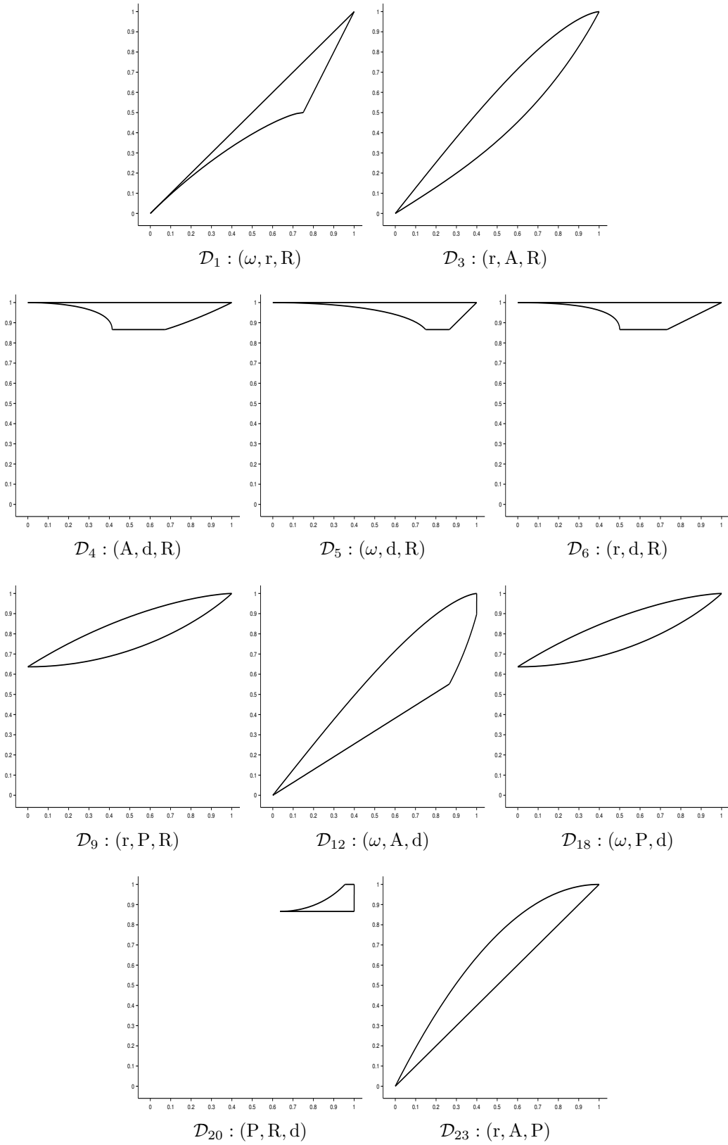
Figure 4: Convex domains of ten shape diagrams for which complete systems of inequalities have been established. For a given shape diagram, the bordered region represents the convex domain in which all compact convex sets lay.
