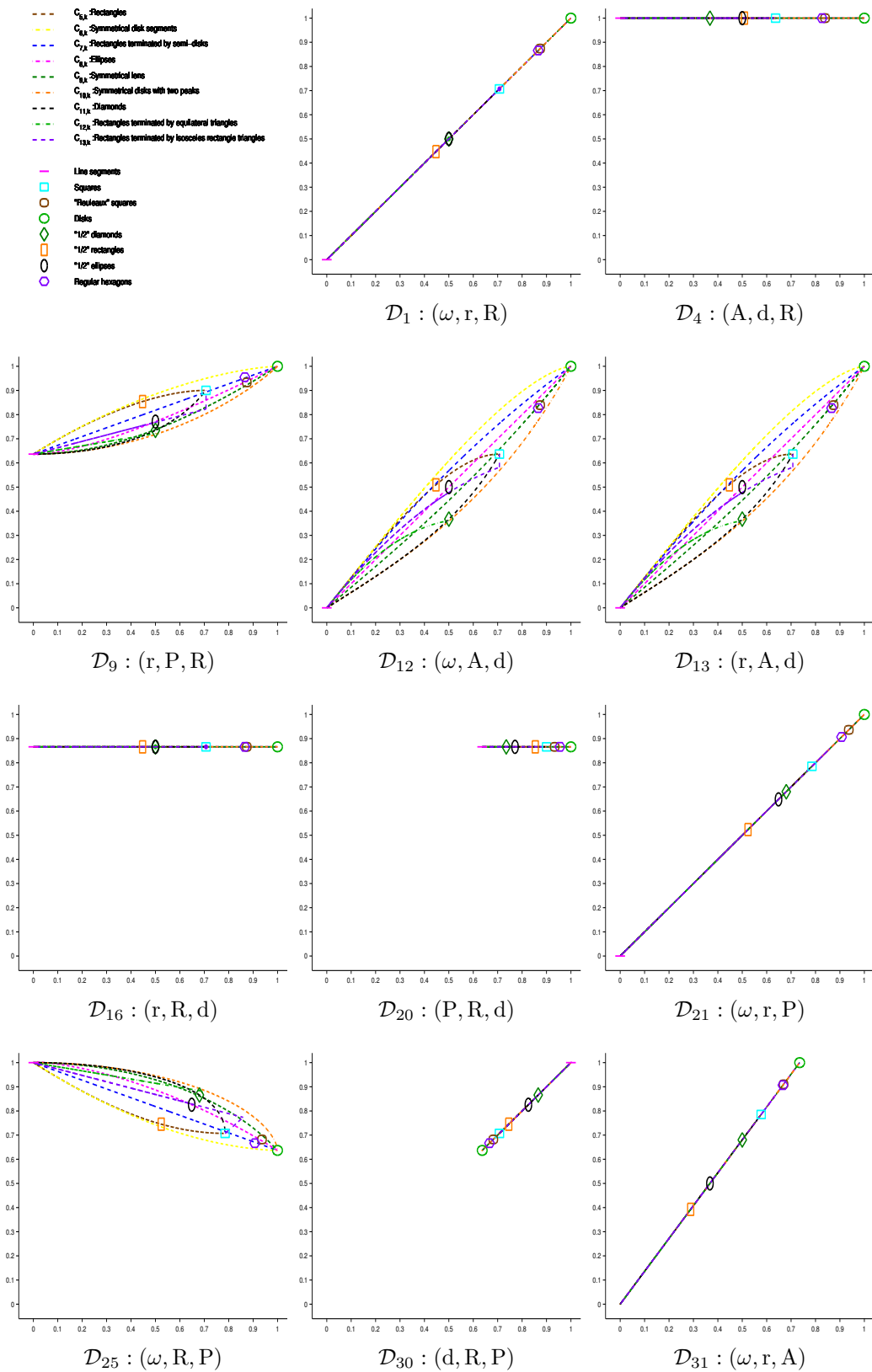
Figure 13: Family \mathcal{F}_{2,2}^c of analytic compact convex sets with one degree of freedom and two symmetrical axes mapped into eleven shape diagrams (chosen according to the results synthesized in section 6).
