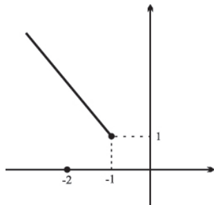
Figure 6: The example of (\Lambda, \sigma \times \tau) -lsc mapping with lower unbounded image
