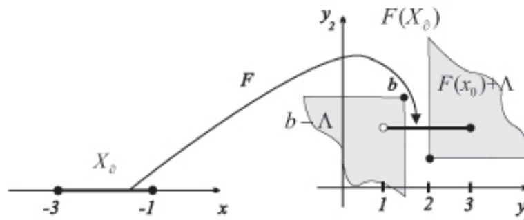
Figure 5: The example of (\Lambda, \sigma \times \tau) -lsc mapping which is neither s -lsc nor q -lsc mapping
