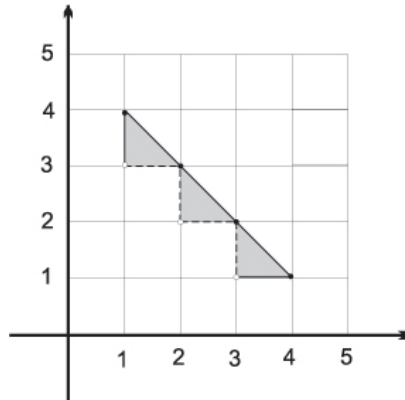
Figure 1: The set S in Example 2.4
