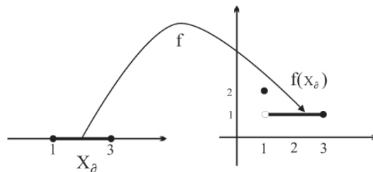
Figure 3: Illustration of Definition 2.9 in Example 2.11
