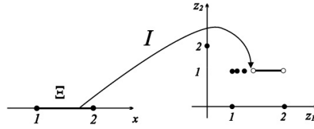
Figure 8: The vector-valued mapping in Example 4.5
