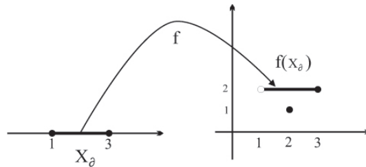
Figure 2: Illustration of the set L_{\min}^{\sigma \times \tau}(f, x_0)
