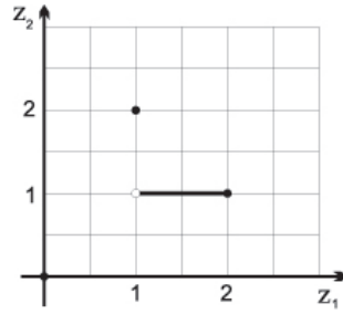
Figure 7: The example of the problem for which \text{Eff}_\tau(X_{ad}; f; \Lambda) = \emptyset
