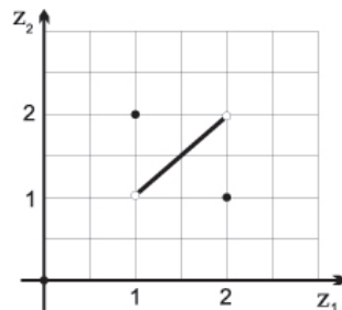
Figure 9: The set f(X_{ad}) to Example 5.6
