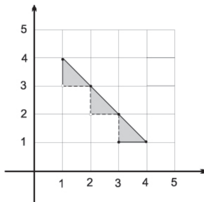
Figure 4: The image of the set X_{ad} in Example 3.4
